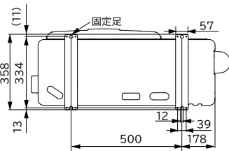
RAC-G56R2・G63R2・G71R2
