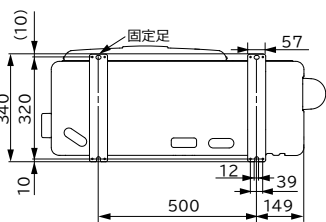
RAC-KG40R2
