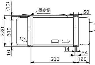
RAC-KG28R・KG36R
