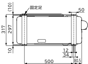
RAC-KG22R・KG25R
