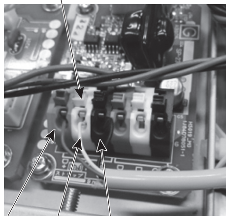
D+ (青) D- (白) GND (黒)
