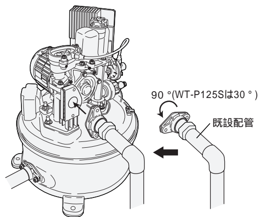
[取付例：WT-P200S]
