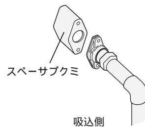
[取付例：WT-P200S]
