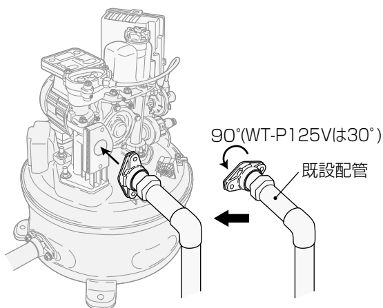
[取付例：WT-P200V]
