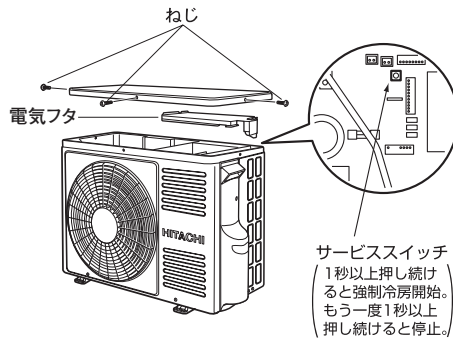
RAC-N40V2
