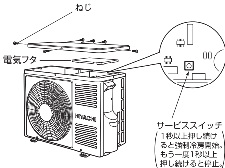
RAC-N28V
