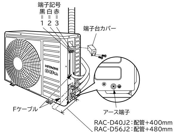
RAC-D40J2・D56J2
